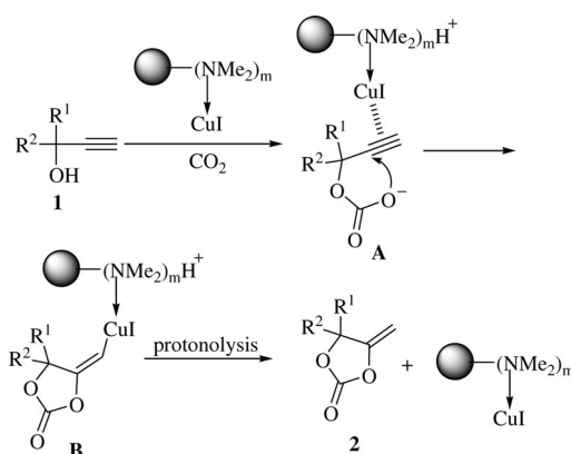
Scheme 2. Proposed mechanism for CO 2 incorporation into propargylic alcohols catalyzed by DMAM-PS-CuI.
